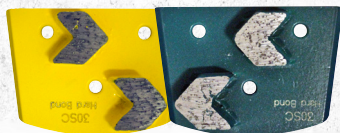
SOFT CONCRETE (Yellow, Left-Hand Arrow, For use on Single & Dual-Disc Grinders) Part # QCAR-SC-0030-L
