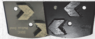
MEDIUM CONCRETE (Grey, Left-Hand Arrow, For use on Single & Dual-Disc Grinders) Part # QCAR-MC-0030
