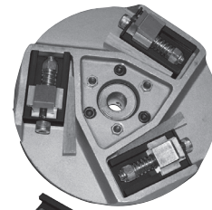
STRIP-SERTS w/MULTI-ACCESSORY DISC
