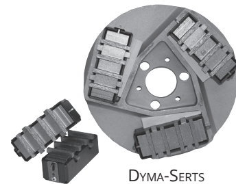
DYMA-SERTS w/MULTI-ACCESSORY DISC
